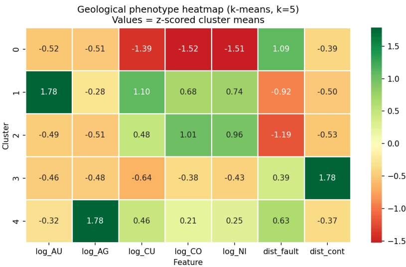
Figure 5. Geological Phenotype Heatmap. Displays z-scored cluster means across geochemical log-minerals and fault distances. This map details the distinct physical characteristics of each phenotype, showing which clusters map to specific mineral enhancements or distinct structural baselines.
