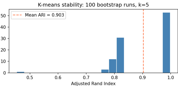
Figure 4. Bootstrap Cluster Stability Histogram. Plots the distribution of Adjusted Rand Index (ARI) scores across 100 independent bootstrap runs on 80% data subsamples. The mean ARI is 0.9027 ± 0.1046, providing clear statistical proof that the K-means cluster structure is robust and stable against sampling noise.
